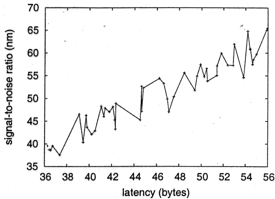
Fig. 5. These results were obtained by Bhabha and Jackson [21]; we reproduce them here for clarity.
