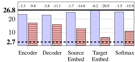
(c) Results on WIPO Ko–En
