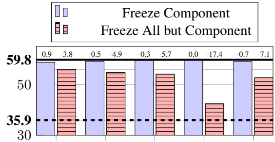
(a) Results on WIPO De–En
