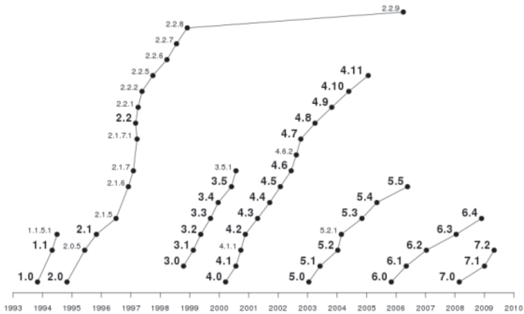
Timeline of the FreeBSD releases. The data for this graph was collected from two sources: the freebsd.org/releases/ which provides month accuracy dates and also the modification time for the the x.x-RELEASE/README.TXT directories. The 2.2.9 release was announce on April 1st, 2006 with a funny message.
