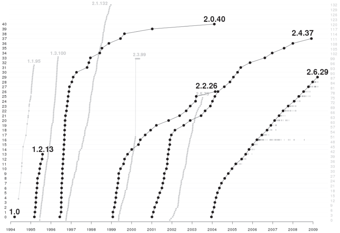
Timeline of the Linux Kernel releases. In gray are depicted the development branches and the small ticks from the the 2.6 branch are the minor releases. The minor that sticks out is the 2.6.16. The data was extracted from the timestamps of the files served by kernel.org. Tho dates, for 2.1.25 and 2.1.26 were wrong and were manually adjusted. The only omitted releases are the 2.2.0pre1 to 2.2.pre9.
