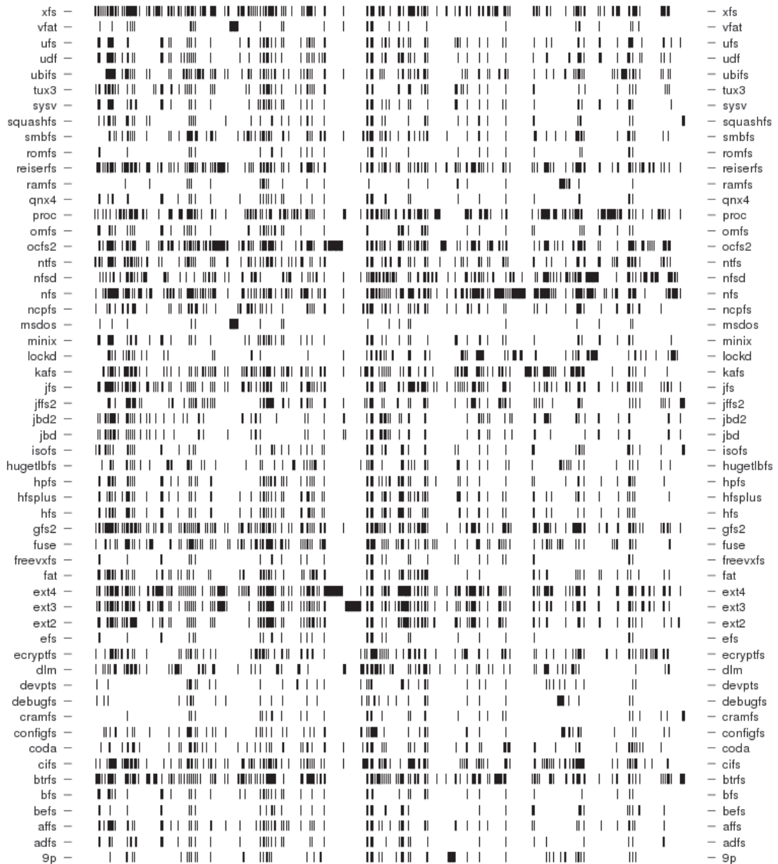
Map of the external symbols. This plot shows the external symbols for 55 kernel modules from the tux3 git repository. Each tick represents an external symbol. The file systems are shown in alphabetical order. The big compact chunks of external symbols related to jbd and jbd2 are visible for ext3 and ext4. The fact that ocfs2 is also making use of jbd2 is also noticeable. Later in this section we will see how this representation looks when is reorganized based on similarities between file systems.
