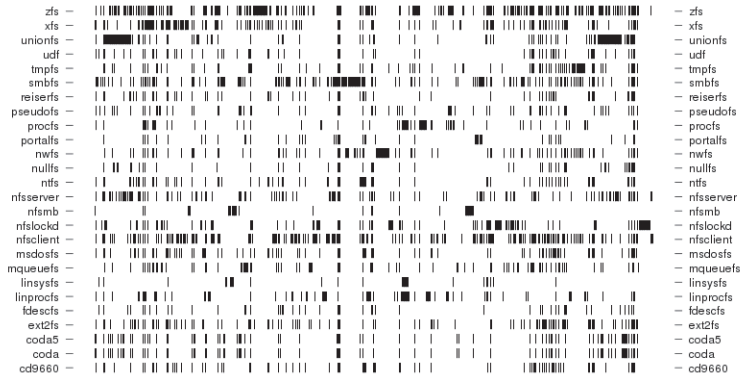
Map of the external symbols for FreeBSD 7.2. As before, each tick represents an external symbol. The horizontal axis contains 832 symbols. The 26 .ko modules related to file systems were taken from the boot/kernel directory of the bootonly install CD. The FFS, the native filesystem for FreeBSD, is not compiled as module so it doesn't show up here.
