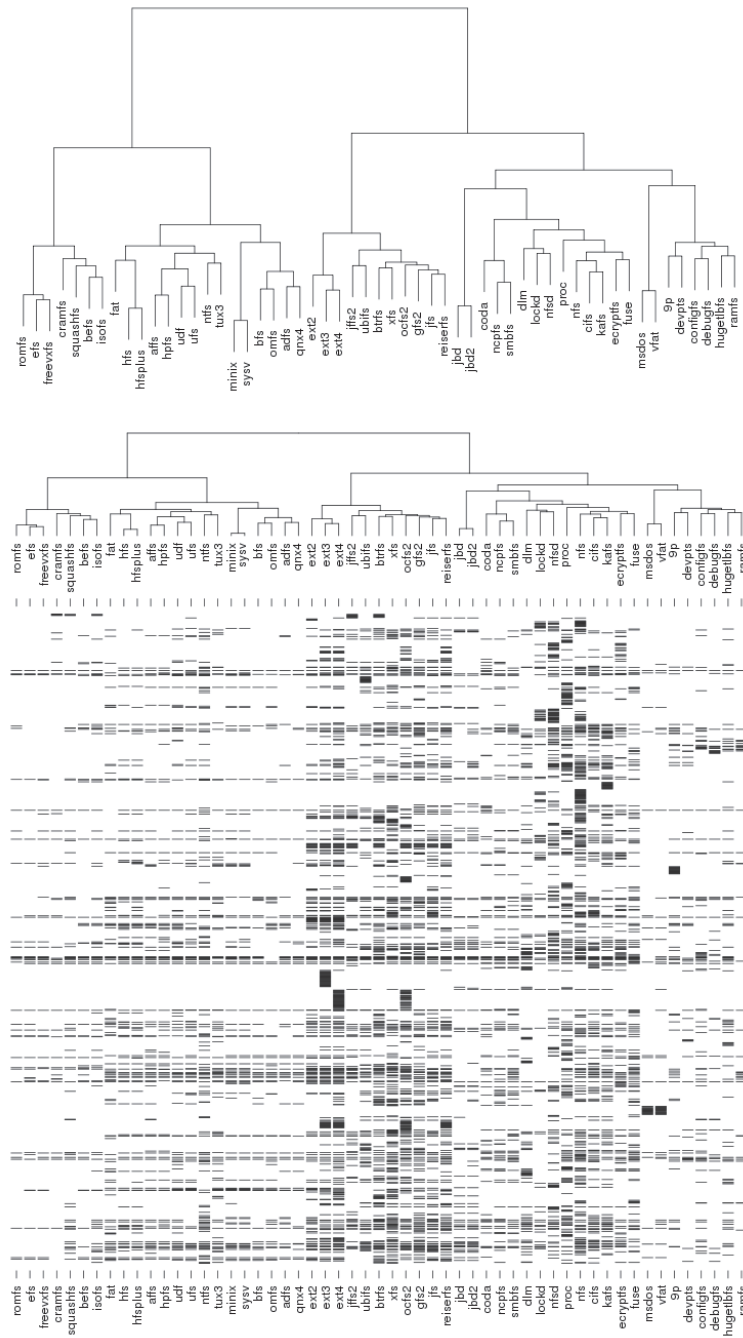
Clustering using the Canberra distance and Ward's method.
