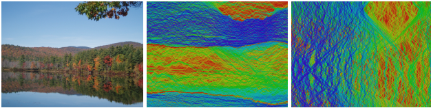
Figure 13: An image with its vertical and horizontal seam index maps \mathbf{V} and \mathbf{H} , colored by their index from blue (first seams) to red (last seams).
