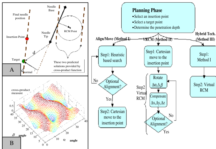
Fig. 3. “A” shows a potential heuristic function, the cross product function. “B” depicts the solution space for all possible cross product values as a function in angles. The chart is illustrating the robot control algorithms using this heuristic information as a feedback. There are three different implementations for this concept: (1) align the needle away from the subject and then move, (2) move to the insertion point and align using VRCM algorithm with small controlled increments, and (3) hybrid technique by combining “1” and “2”, where we “first” align-move and “second” enhance the result by running VRCM.
