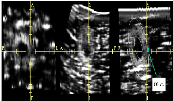
Fig. 4. Orthogonal slices of 3DUS reconstruction of an olive in calf liver phantom.
