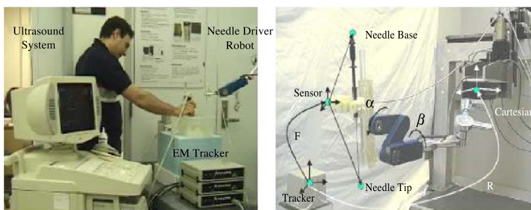
Fig. 2. Physical setup. (A) Illustrates the setup during freehand 3DUS capture. (B) The needle driver robot is comprised of a 3-DOF Cartesian stage, a passive unencoded adjustable arm, a 2-DOF motorized rotational stage, and a magnetic tracker attached to the tool holder.
