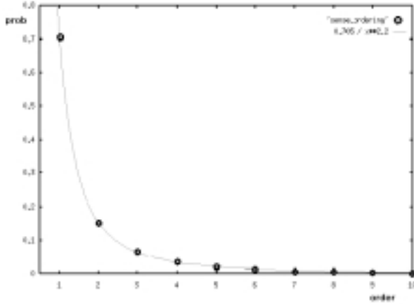
Figure 2: Sense distribution in SemCor
