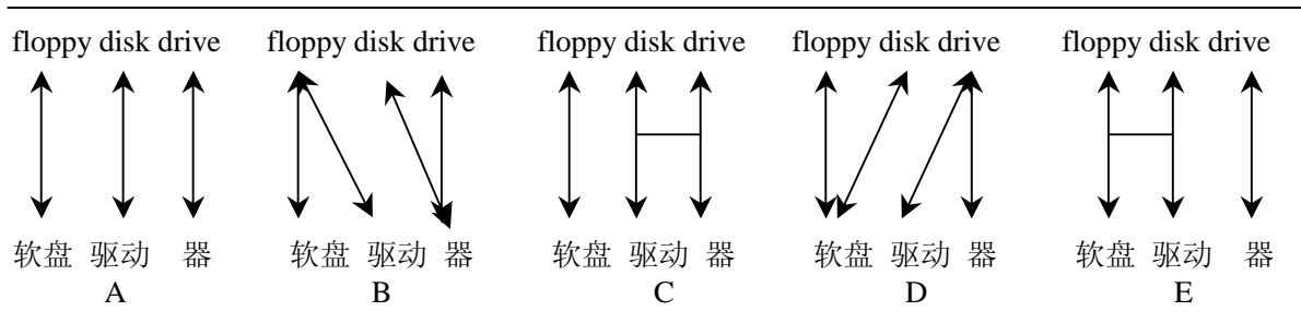
Figure 3. The Possible Word Alignment Forms in One Chunk
