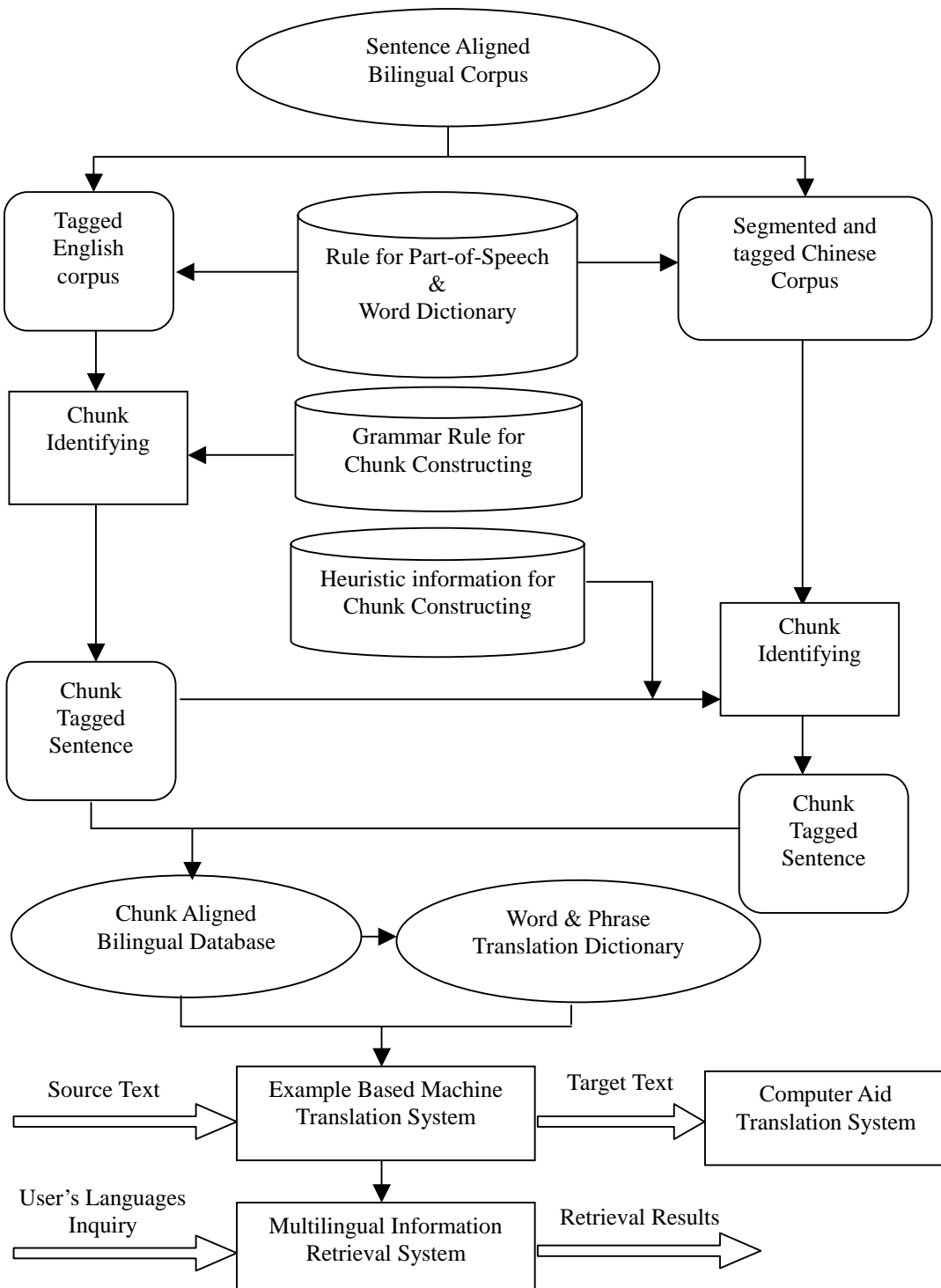
Figure 4. System Architecture
